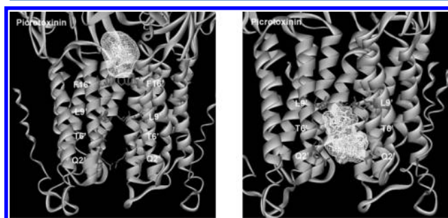
Figure 5. Overlay of 10 docked poses for PXN in the ELIC pore. The channel is seen from the side, and the ligands are located above F16' (left) or close to the residues at position 6' (right).
