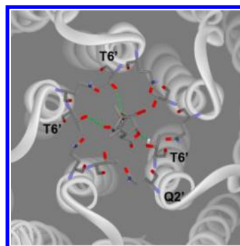
Figure 6. Example docked pose for PXN in the ELIC channel. PXN is located close to the Thr residues at position 6', where it is stabilized by hydrogen bonds. The channel is seen from the top looking down toward the cell interior.
